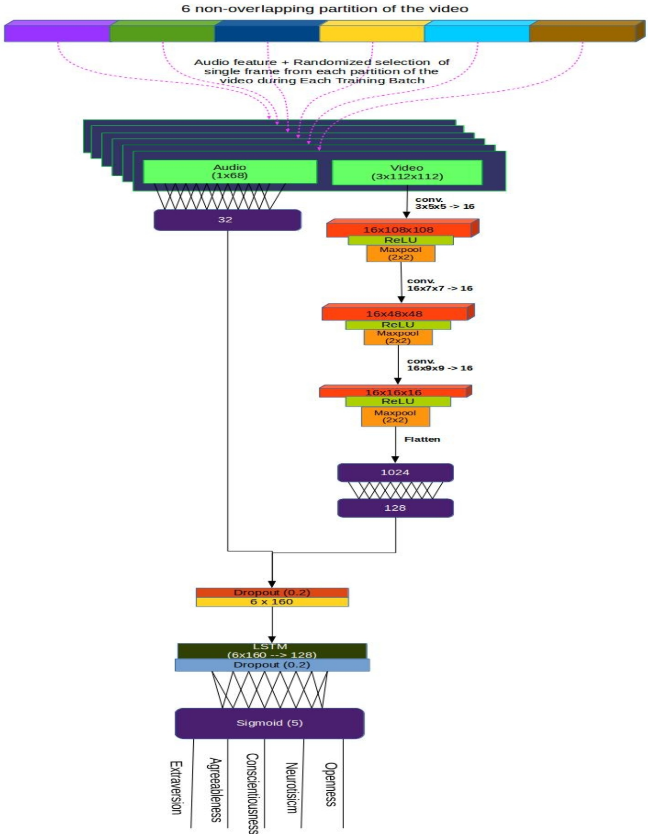
Figure 1: Multi-modal LSTM Neural Network architecture
